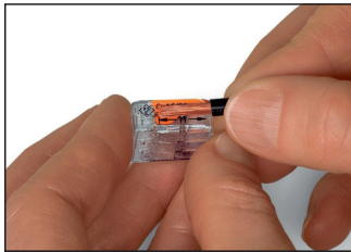
Strip conductor to 11 mm Pelar el conductor a 11 mm
